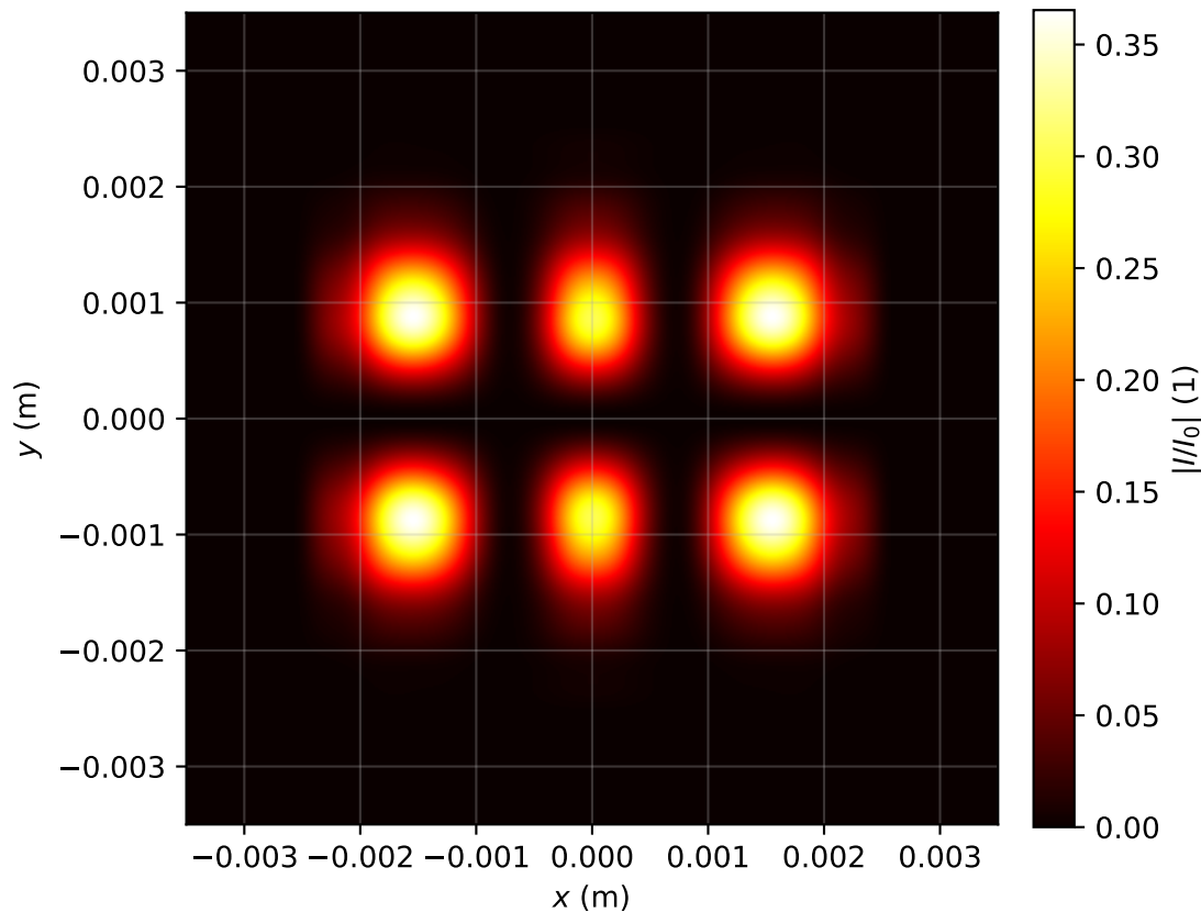
Intensity profile I(x, y, z = 3.344)/I_0 , P_{in}=2.0P_{cr} , artificial time
